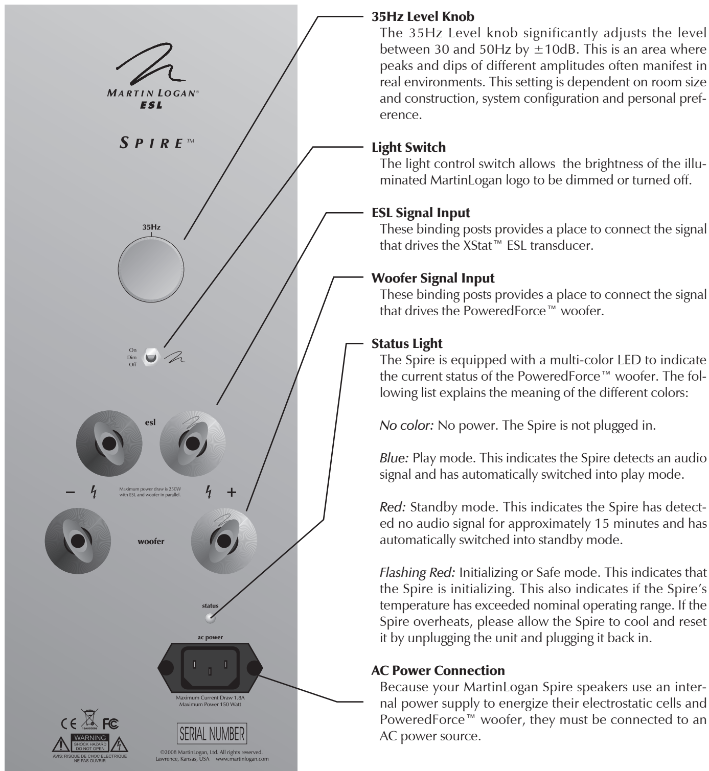
Figure 1. Spire Controls and Connections
