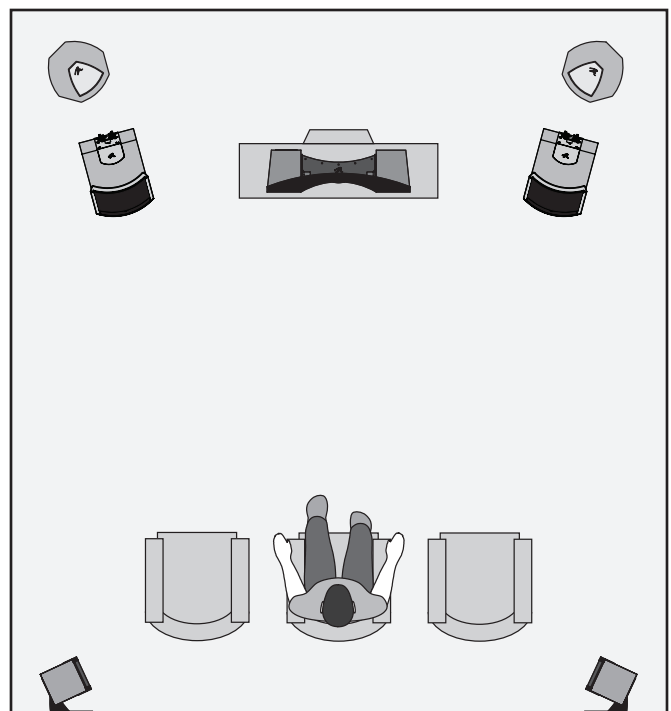
Figure 12. Spire speakers as front channels, the Stage as the center and surround channels, and Descent i subwoofers as 0.1 (effects) channel.
